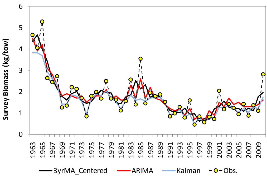
Figure 4. Observed NEFSC fall survey biomass(kg/tow) time series with 3 year-centered point moving average, ARIMA and Kalman filter time series fit for southern silver hake, 1963-2010.
